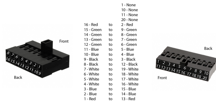
1C, 26AWG, 30 cm long 3014 - Wire Assembly for LCDs with 2x8 Pinout
